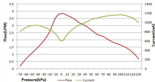
AJK-B06A4002 Flow(LPM) & Current(mA)
